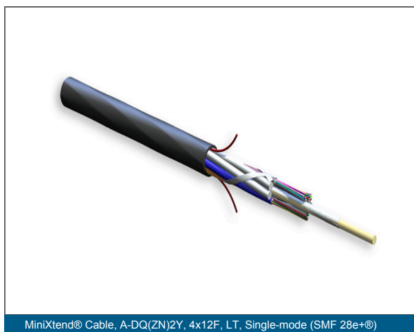
MiniXtend® Cable, A-DQ(ZN)2Y, 4x12F, LT, Single-mode (SMF 28e+®)
